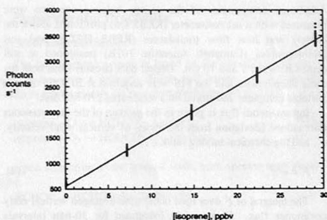
Figure 2. Calibration data for FIS sensor. Sample flow = 3.46 SLPM, O_2 flow rate = 0.80 SLPM, ozone partial pressure = 25 Torr, sampling rate = 1 Hz, time at each mixing ratio ~45 s, slope = 98.2 \text{ photons s}^{-1}/(\text{ppbv isoprene})^{-1} , intercept = 556 \text{ photons s}^{-1} , R = 0.997 .
