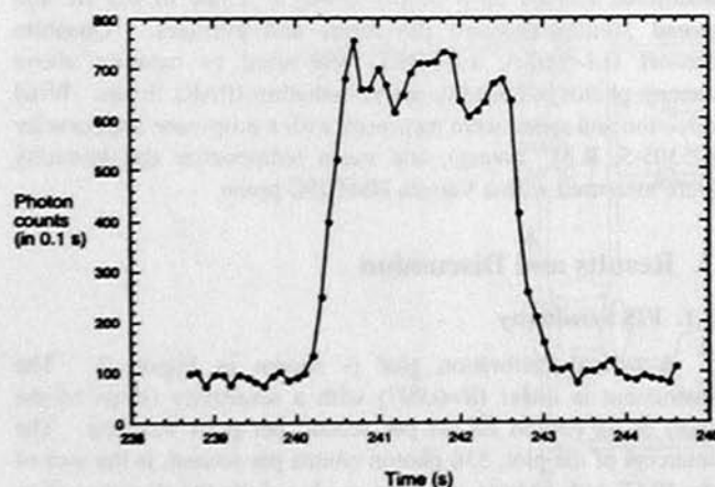
Figure 3. Response time characteristics for FIS sensor. Flow rates and ozone mixing ratio match those of Figure 2.
